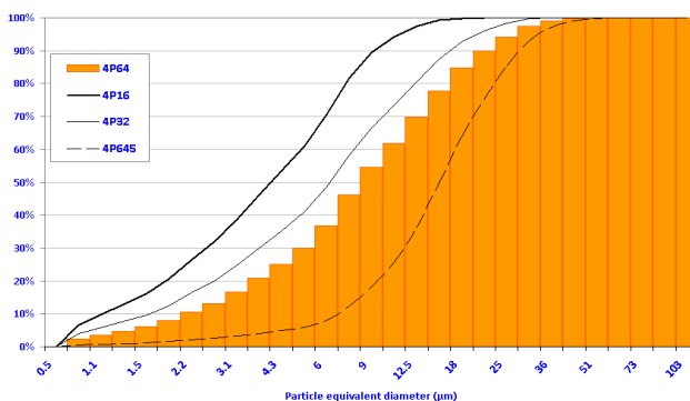
4P64 - Cumulative size distribution on log scale
