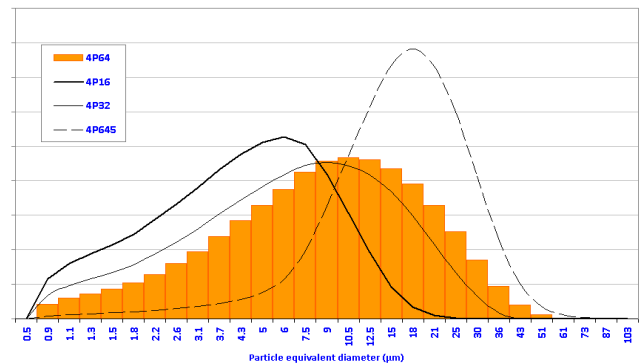
4P64 - Size distribution on log scale
